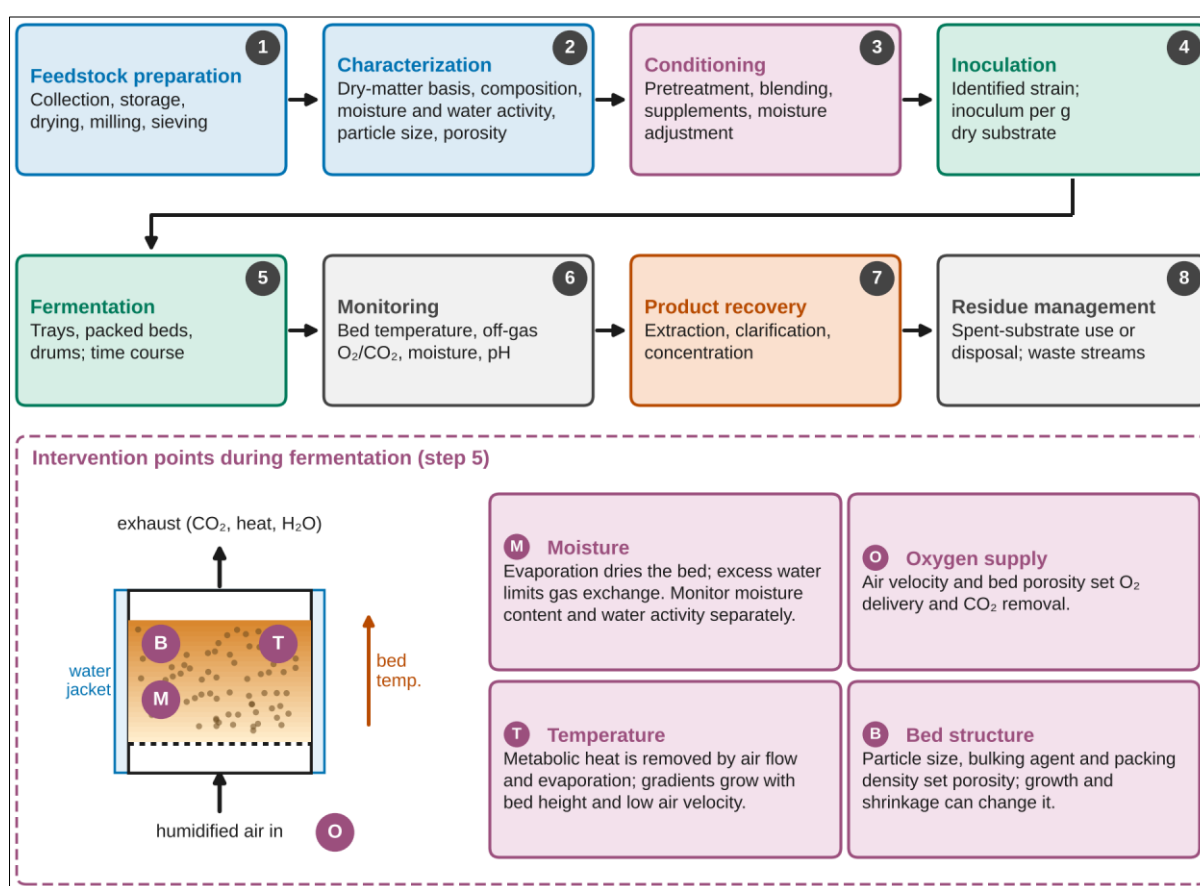
Fig 2: Solid-state fermentation process (steps 1–8) and intervention points during fermentation: M, moisture; O, oxygen supply; T, temperature; B, bed structure. The packed-bed drawing is schematic, with forced aeration and a water jacket; the shading indicates that bed temperature can rise along the airflow path when heat removal is inadequate (Mitchell et al. , 2023; Sentís-Moré et al. , 2023). O 2 , oxygen; CO 2 , carbon dioxide.
