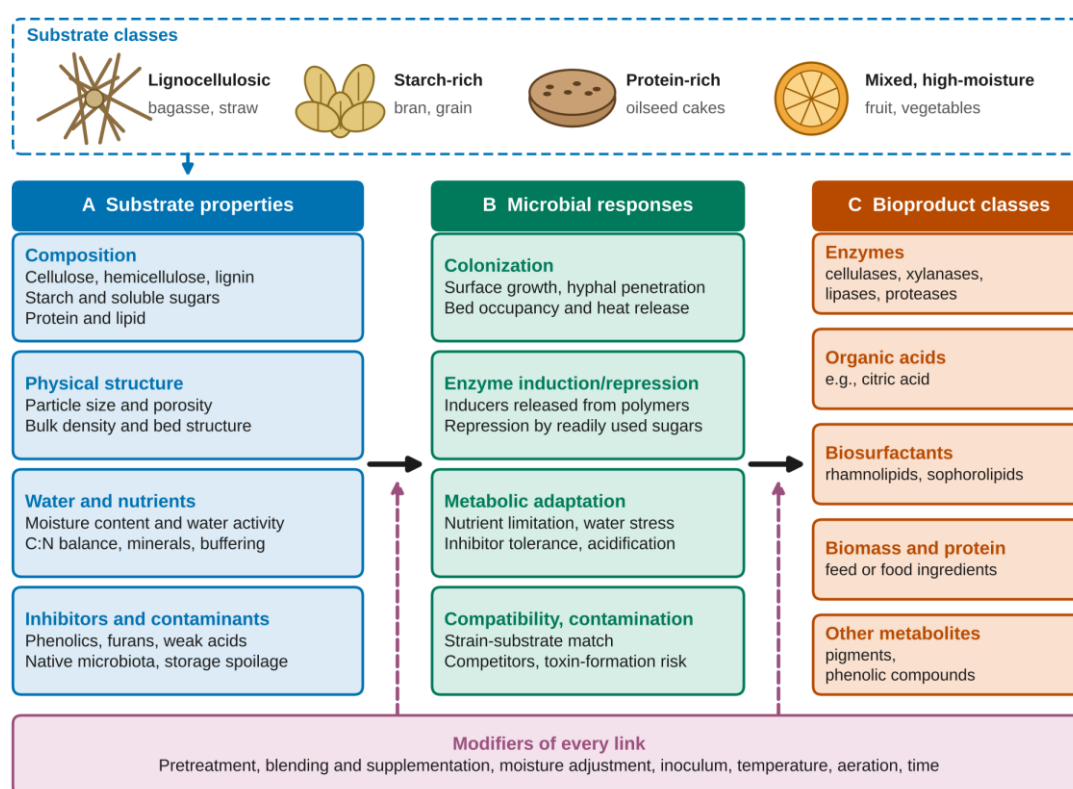
Fig 1: Conceptual framework linking substrate properties (A), microbial responses (B) and bioproduct classes (C) in solid-state fermentation. Solid arrows show the direction of influence synthesized in this review; dashed arrows show that pretreatment, blending, moisture adjustment, inoculum and process conditions modify each link. Substrate icons are schematic. Relationships are drawn from the studies discussed in Sections 3–6 (e.g., Astudillo et al. , 2023; Borkertas et al. , 2025; Costa et al. , 2023; Nargotra et al. , 2023) [2, 3, 7, 17] and represent qualitative associations, not quantified effects. C:N, carbon-to-nitrogen ratio.
